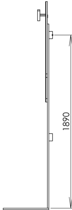
Spegel/Mirror/Peili
